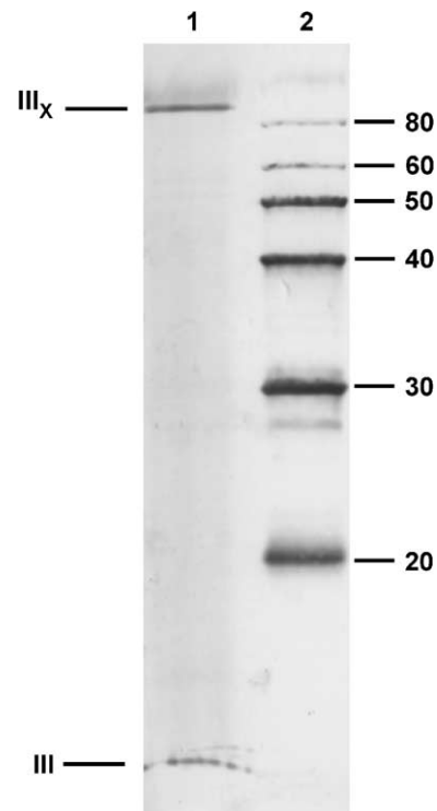
Fig. 6. Immunoblot of the chloroplast ATP synthase oligomer III from C. reinhardtii . Solubilized ATP synthase (lane 1) and a molecular weight marker (kDa) (lane 2) were transferred to a PVDF membrane and then incubated with polyclonal antibodies raised against the chloroform extracted monomer III from spinach.
